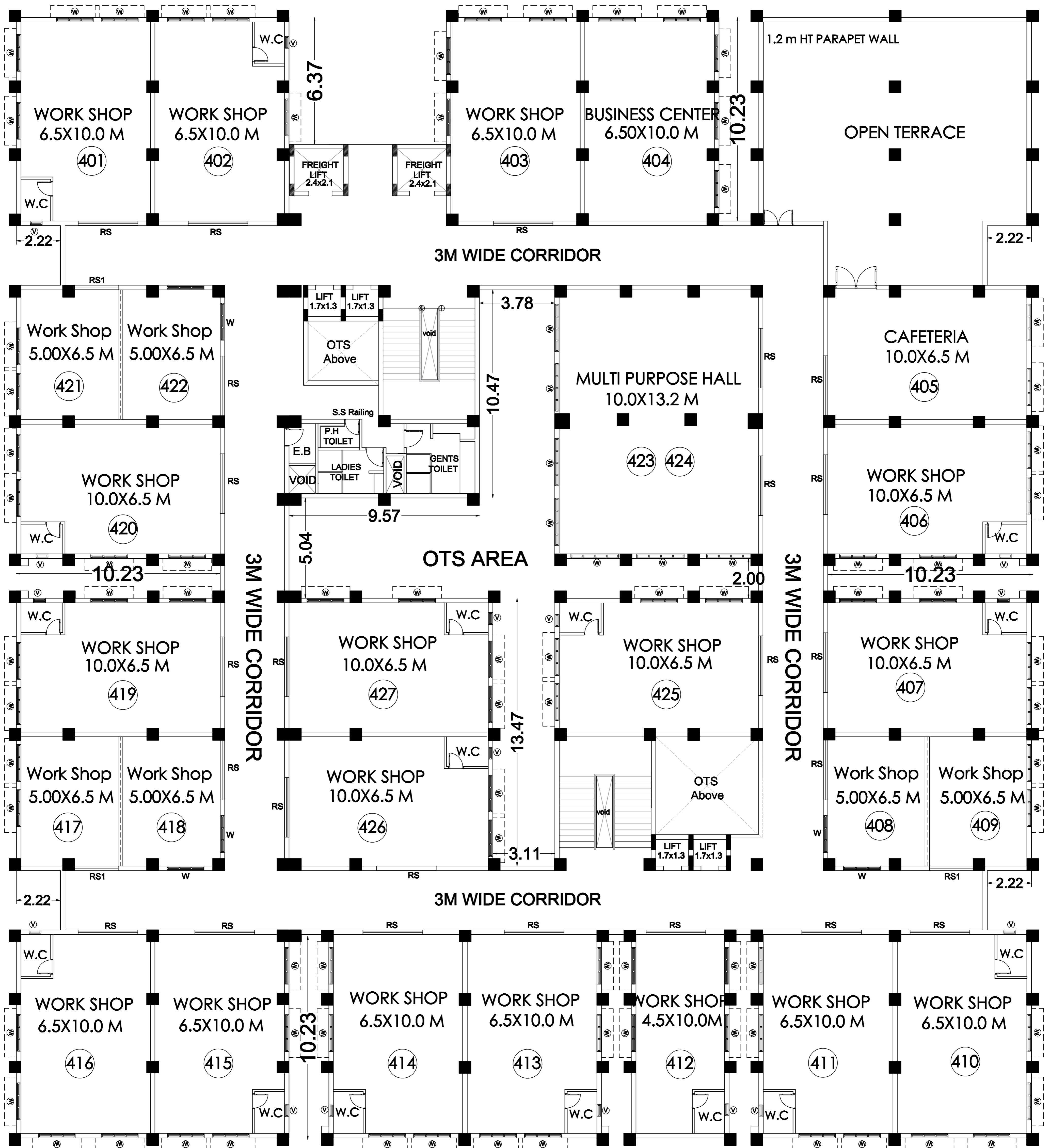
FOURTH FLOOR PLAN
